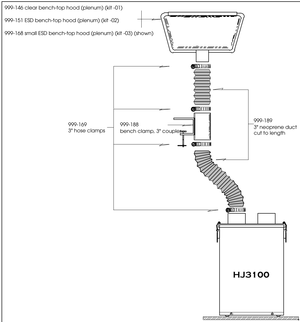
999-206-xx Bench top hood kit
