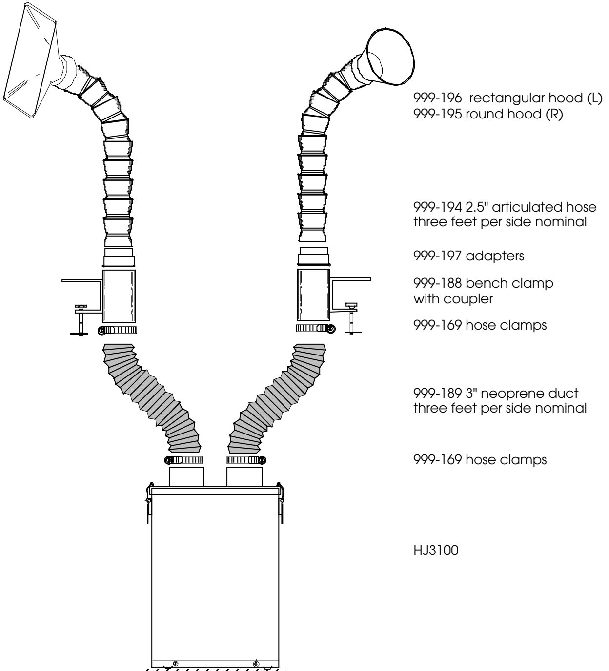
Figure 5. Using articulated ESD-safe hose and hoods.
