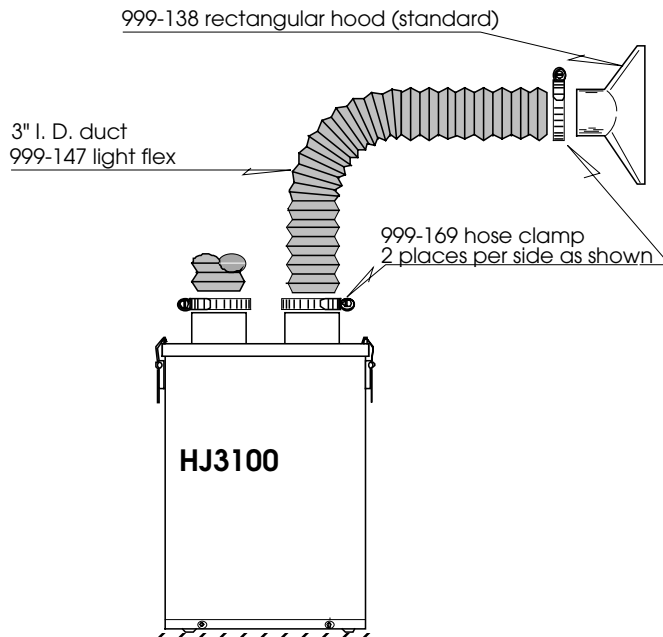
Figure 3. Basic HJ3100-02 installation. One side shown.
