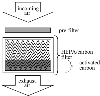
Figure 1a The standard Hakko filter.
