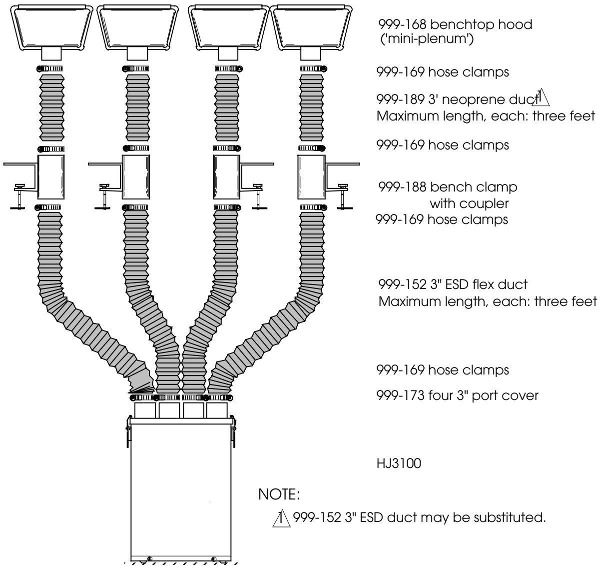
Figure 6. Typical installation - four port cover.
