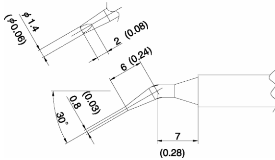
T7-JD16 SHAPE-1.6JD
