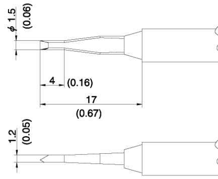
T7-SBS04 SHAPE-0.4SBS
