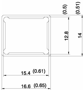
T7-1210 PLCC 15.4×12.8
