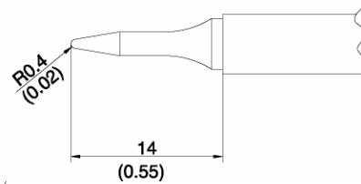
T7-SBS07 SHAPE-0.7SBS
