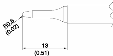
T7-SBS07 SHAPE-0.7SBS
