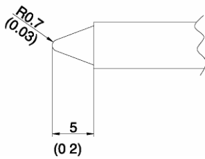
T7-B4 SHAPE-0.4B
