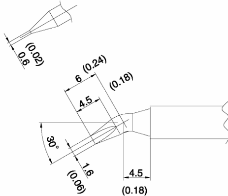
T7-JD16 SHAPE-1.6JD
