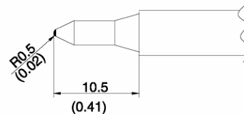
T7-SB08 SHAPE-0.8SB
